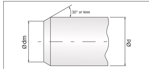
Fig. 6 : Shaft lead-in chamfer
