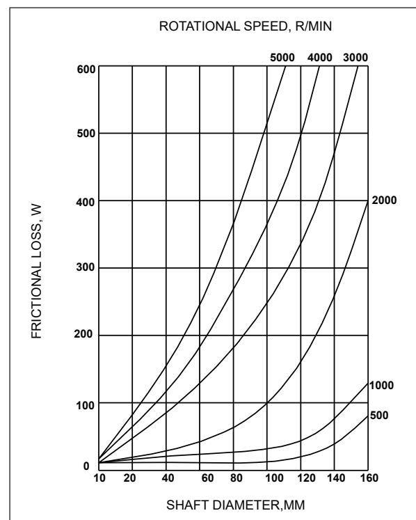
Fig. 7 : Frictional loss for standard NBR oil seal
