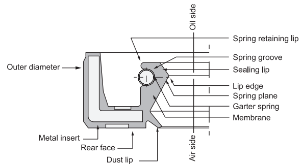
Fig. 1 : Rotary shaft seal nomenclature
