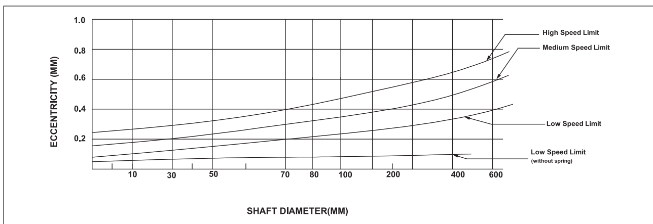
Fig. 5 : Shaft eccentricity limits
