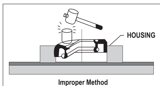
Installation aids for fitting rotary shaft seals
