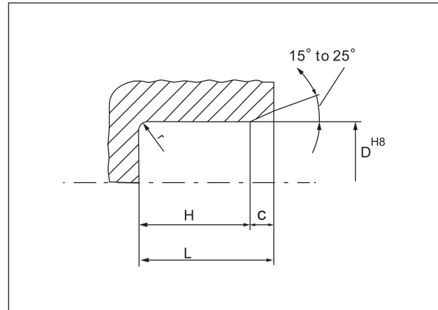
Fig. 9 : Housing drawing with depth and chamfer.
