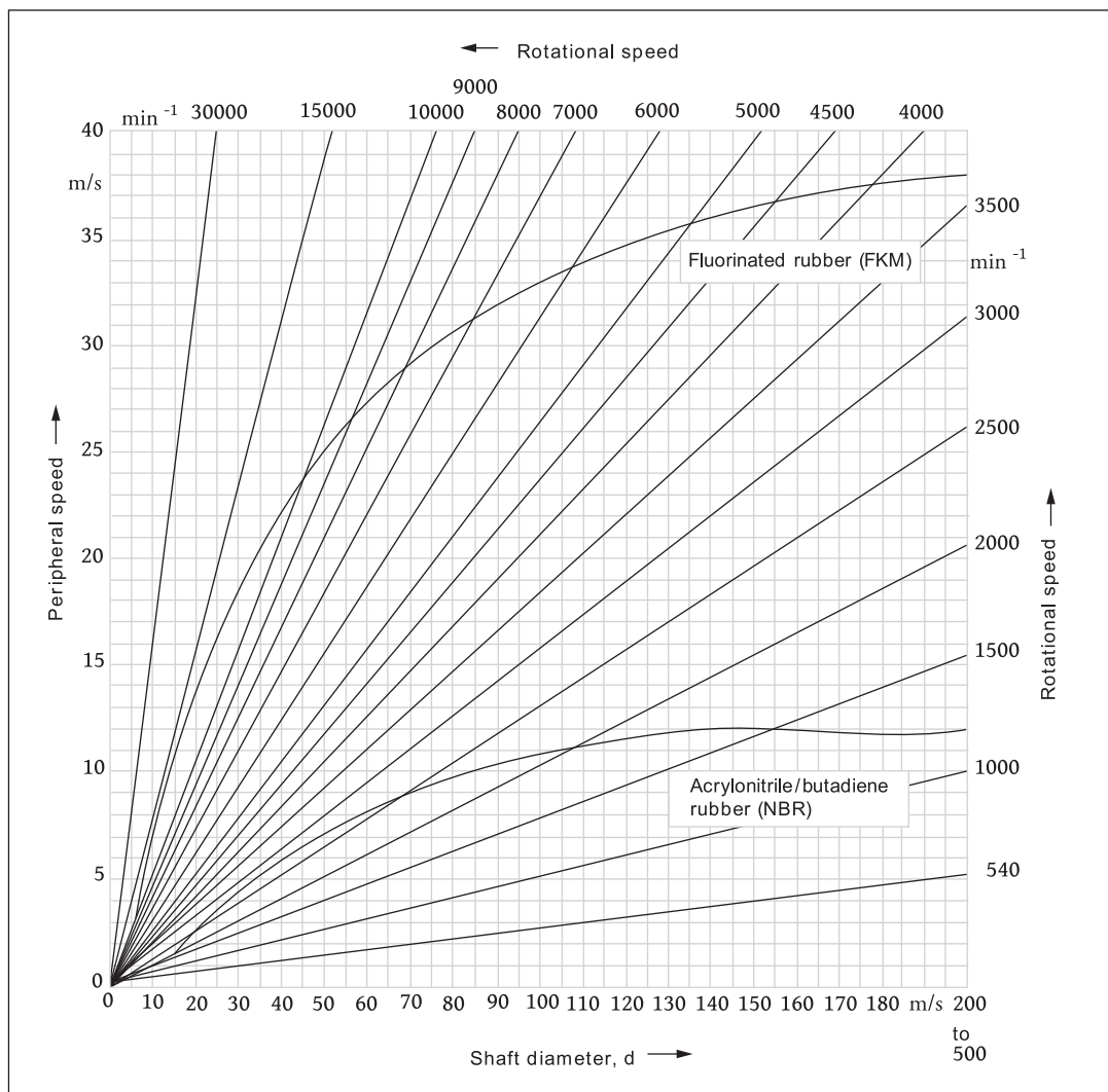
Fig. 5 : Maximum permissible rotational speed for unpressurised operation.
