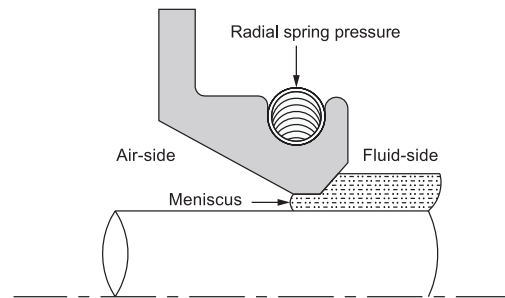
Fig. 2 : Sealing lip design
