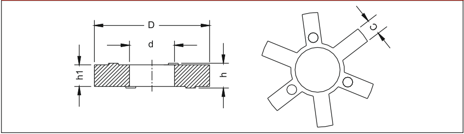
Model No. N = NBR Spider, P = PU Spider (Sizes in mm)
